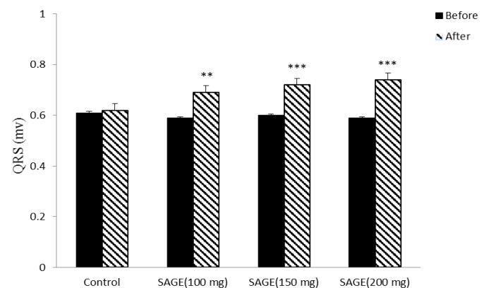
Figure 1: Effect of Sage (100, 150 and 200 mg/kg) on voltage of QRS complex in rats. Results were expressed as Mean ± SEM of 8 rats per group, used t-test; **P<0.01, ***P<0.001.
